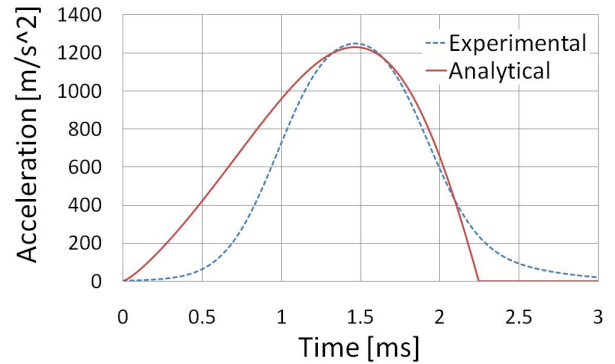
Figure E.2 Comparison of experimental and analytical accelerations for the medium impactor from a 12" drop.
