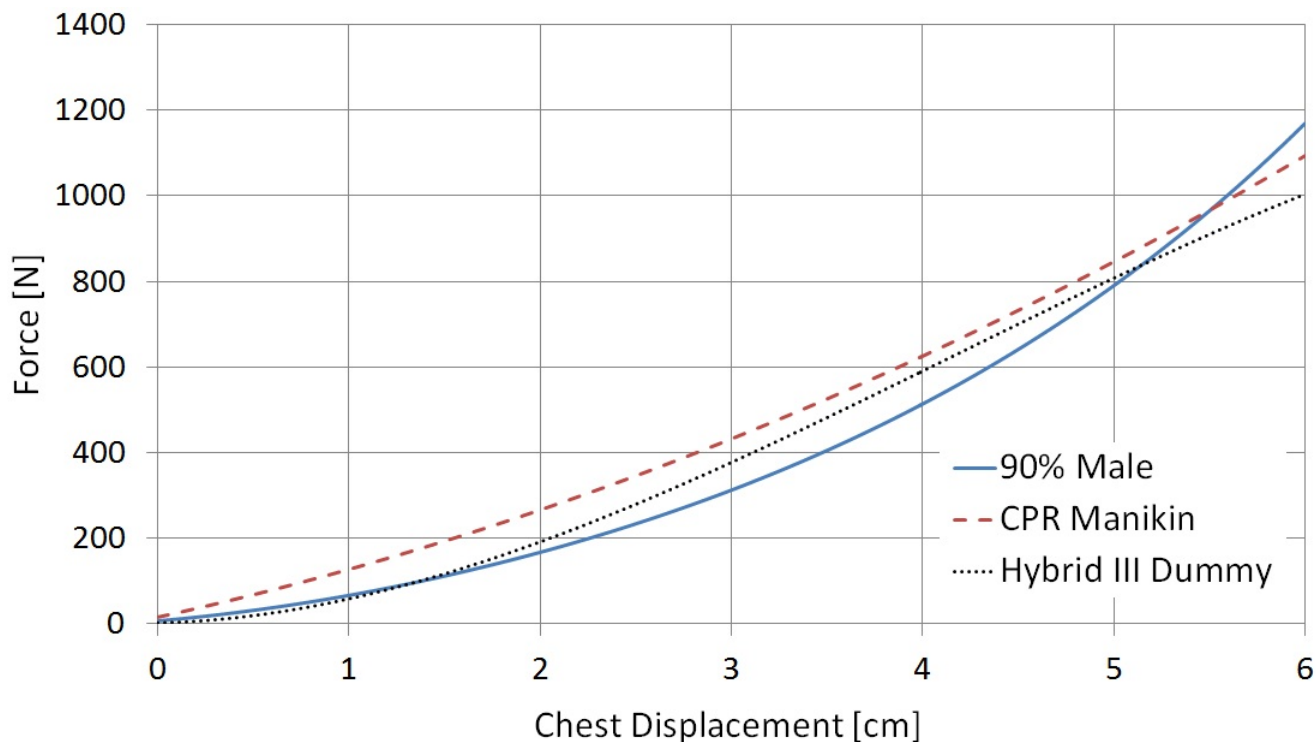
Figure 3.4 Chest deflection for 90% male, CPR manikin, and hybrid III dummy for comparison.
