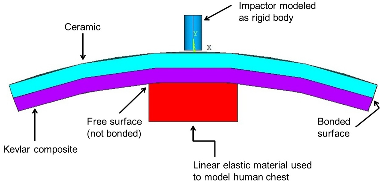
Figure 3.5 Ansys model.
