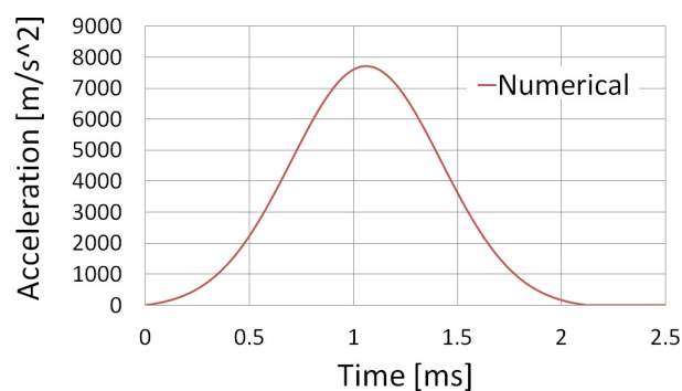
Figure A.14 Numerical acceleration for the small impactor from a 72" drop.
